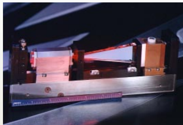
Alternative example of diode-pumped solid-state laser development pursued by the research team. Developed at Livermore by Eric Honea and his collaborators, this laser, with a 2-micrometer thulium-doped yttrium–aluminum–garnet laser head, achieved power levels nearly ten times greater than those previously possible.
