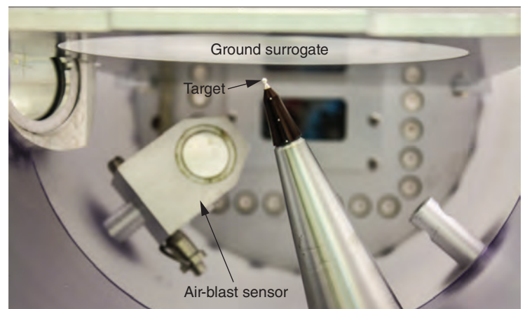
(top) In the energy-partitioning, energy-coupling (EPEC) experiments at the National Ignition Facility (NIF), a diagnostic instrument manipulator inserts a pressure cylinder into NIF’s 10-meter-diameter target chamber. (bottom) The photo shows the cylinder with a target, air-blast sensor, and ground surrogate installed.
