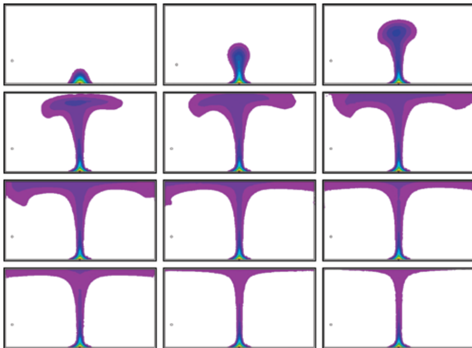
Groundwater modeling was used to simulate a hypothetical contaminant transport scenario in a subsurface homogeneous aquifer above a UCG coal seam. The model couples flow, heat, mass, and density to calculate changes in the temporal and spatial distribution of contaminants generated by the gasification process. In this simple case, the heat and contaminant sources are modeled for a stationary ignition point, and groundwater flow rates are minimized to highlight the buoyancy effects on the contaminant plume. The contaminant concentrations over time, from top left to bottom right, are shown (purple is lowest, red–yellow is highest).
