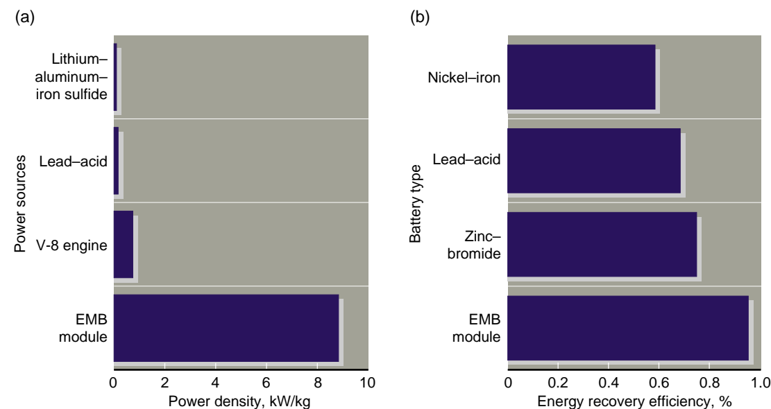
Figure 5. Various energy storage devices are compared for (a) power density and (b) energy recovery.
