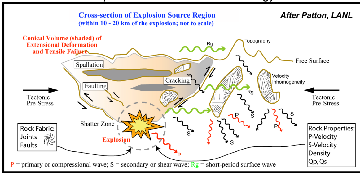
Figure 2. An illustration showing many potential sources of explosion S-waves created as the initially spherically symmetric pure P-wave explosion interacts with emplacement rock and the free surface of the Earth (after Patton, written comm.).
