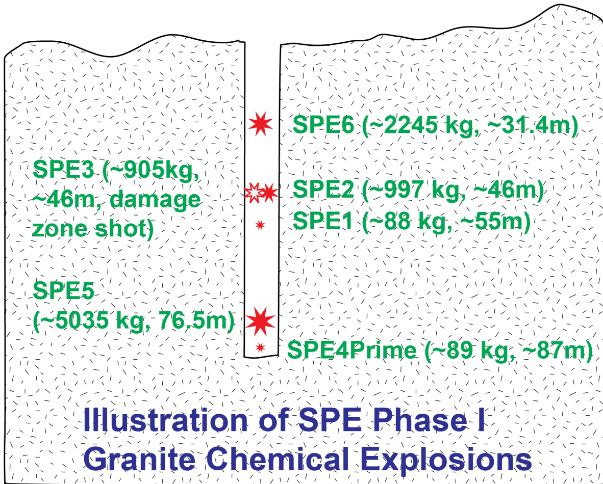
Figure 3. Illustration of relative size, depth and order of the Phase I shots in the granite hard rock hole on Climax Stock. Shots carried out to date indicated in green. Details for each shot are given in the Table 1.
